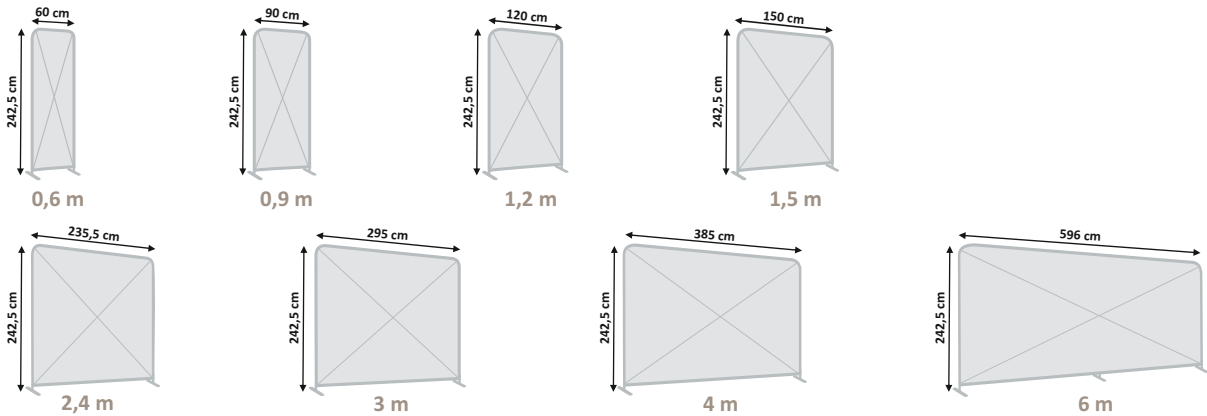
ZIPPER WALL STRAIGHT
